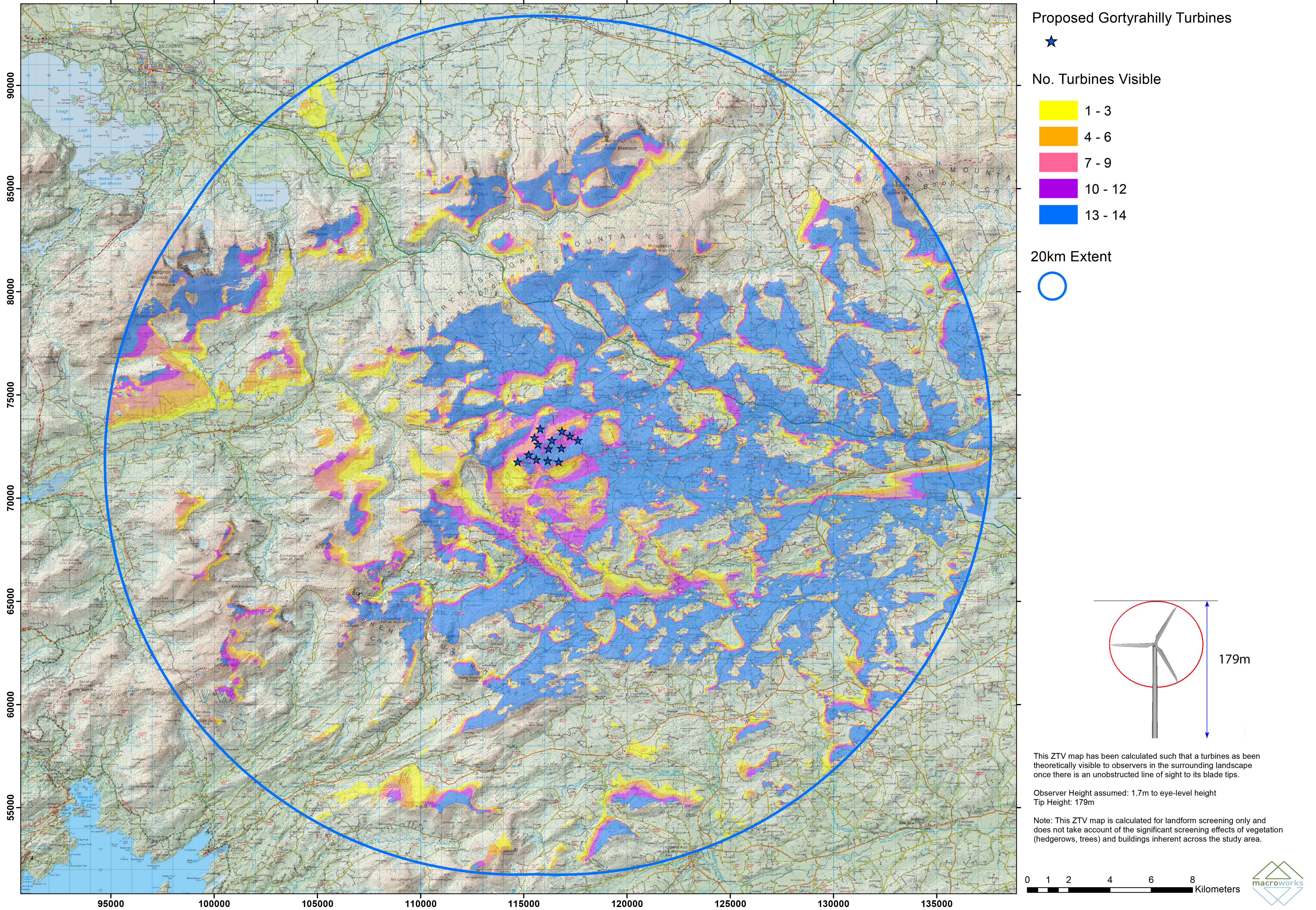
Figure 12.3 ZTV (Zone of Theoretical Visibility) indicating the areas that have a potential view of Gortyrhilly Wind Farm turbines at 179m Tip Height
